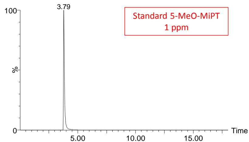
Figure 3B. Identification of 5-MeO-MiPT in Corazon pill. HE spectra (left) and chromatographic peak (right) obtained for the suspect compound in the sample extract (top) and for 5-MeO-MiPT reference standard (bottom).
