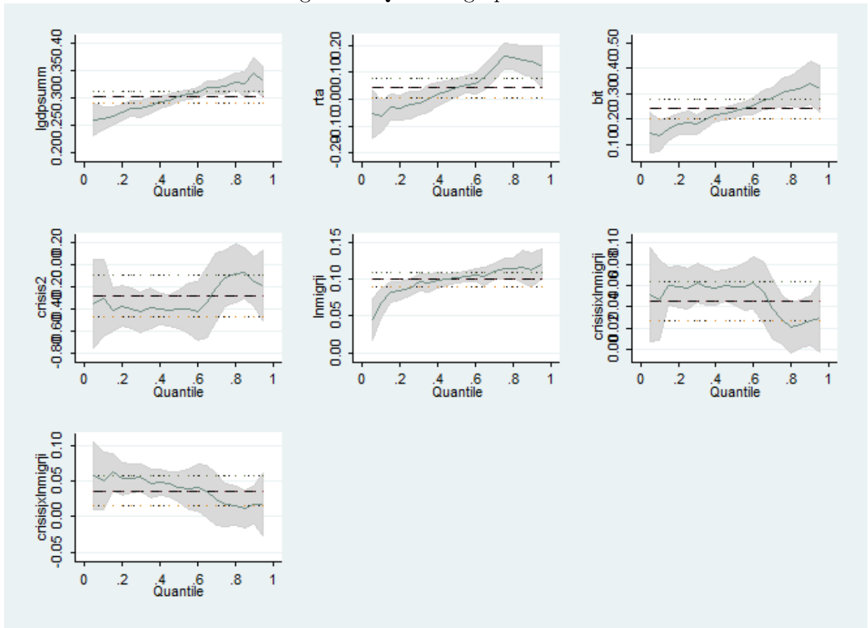
Figure 1: Quantile graphs
