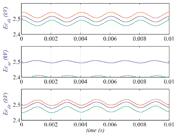
Fig. 16. Average, maximum and minimum cell capacitor voltages in shunt, series and derivation branches when delivering 600MW.
