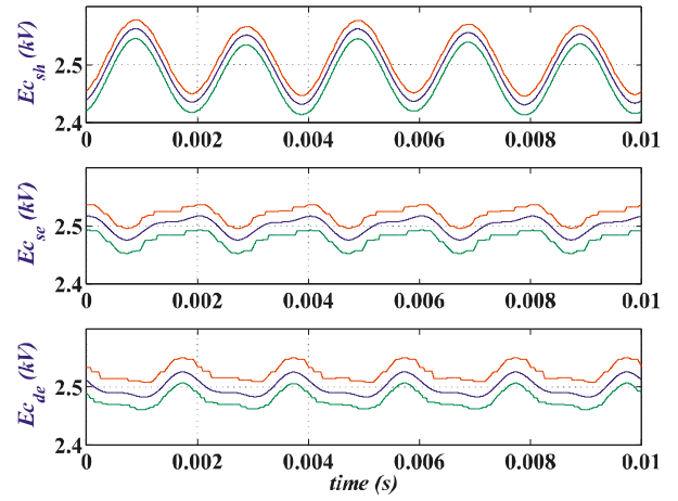
Fig. 8. Cell voltages when delivering 200MW.
