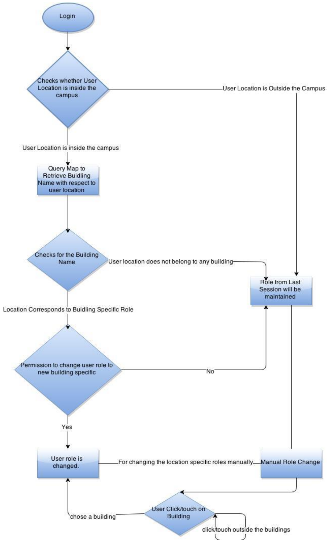
Figure 12: Decision Tree for assigning location-specific role
