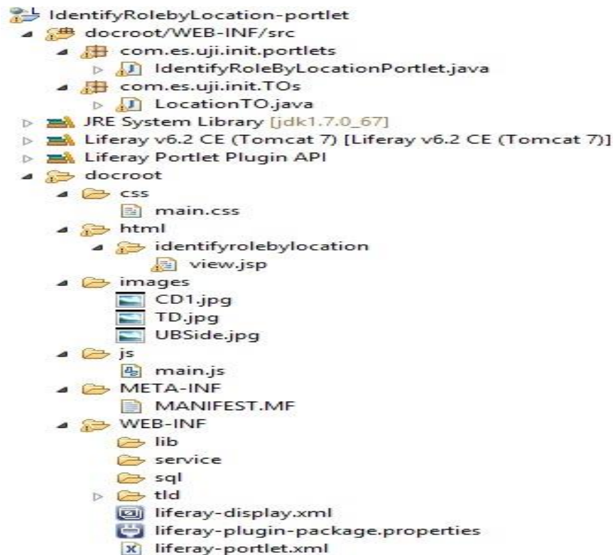
Figure 14: Example structure of Portlet Plugin
