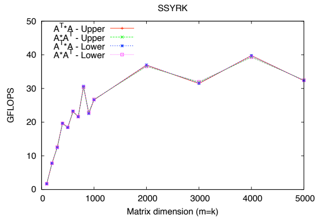
Figure 3. Performance evaluation for the implementation of SSYRK in CUBLAS
