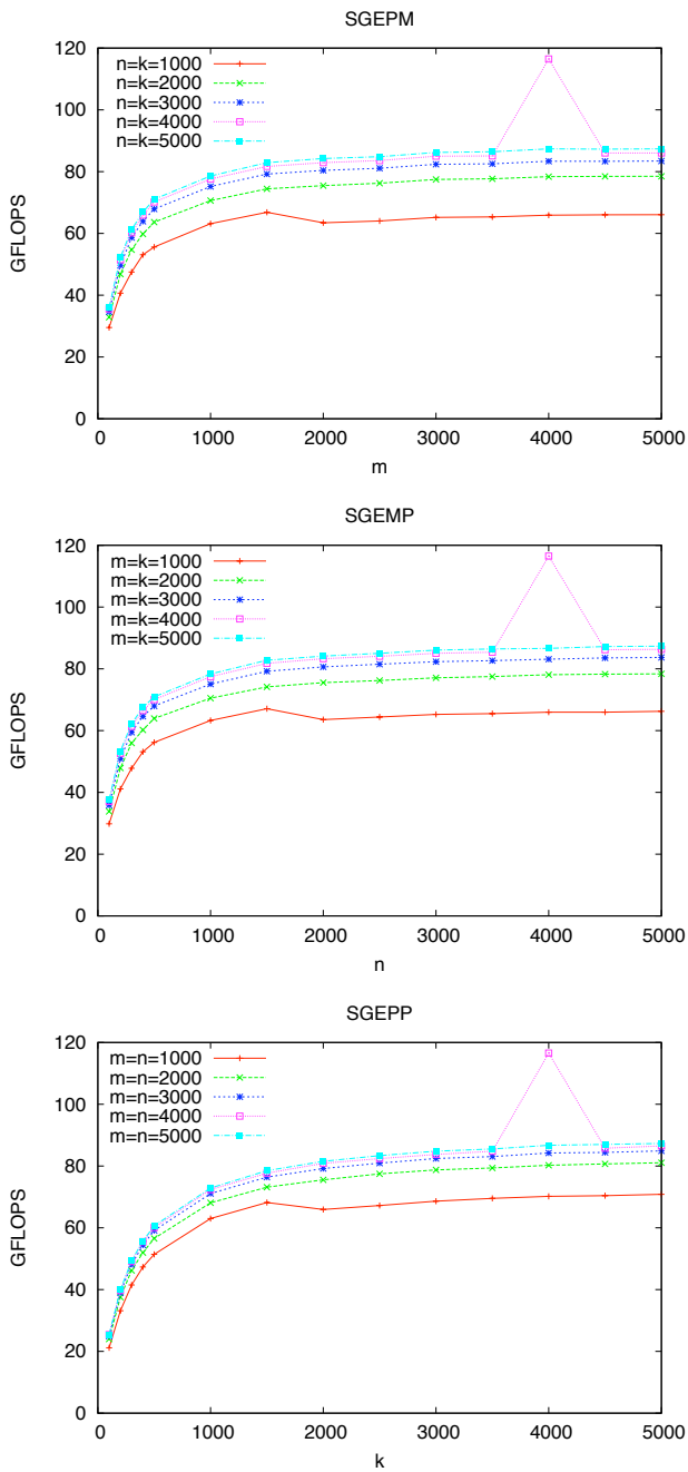
Figure 2. Performance evaluation for the “implementations” of SGEPM (top), SGEMP (middle), and SGEPP (bottom) in CUBLAS, used to compute the matrix multiplication C := C + AB ; two dimensions fixed
