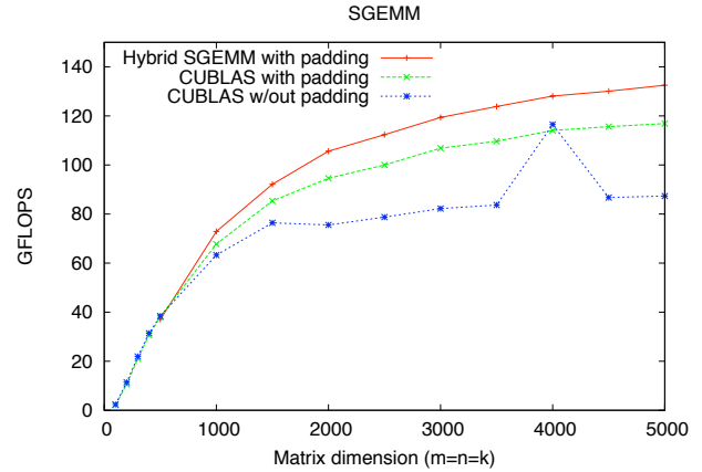
Figure 13. Performance evaluation for the implementation of _{SGEMM} in CUBLAS, the implementation of _{SGEMM} with padding, and the hybrid implementation of _{SGEMM} (with padding)
