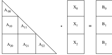
Figure 9. Decomposition of the STRSM operation to build it on top of SGEMM
