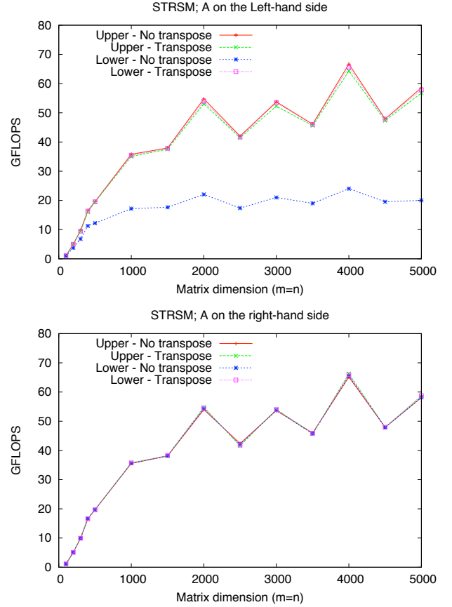
Figure 5. Performance evaluation for the implementation of STRSM in CUBLAS with A to the left-hand (top) or right-hand (bottom) side of the unknown matrix
