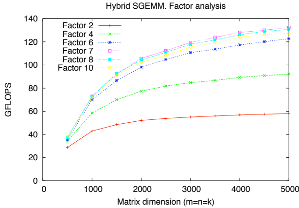
Figure 12. Impact of the partition sizes over the performance of the hybrid _{SGEMM}
