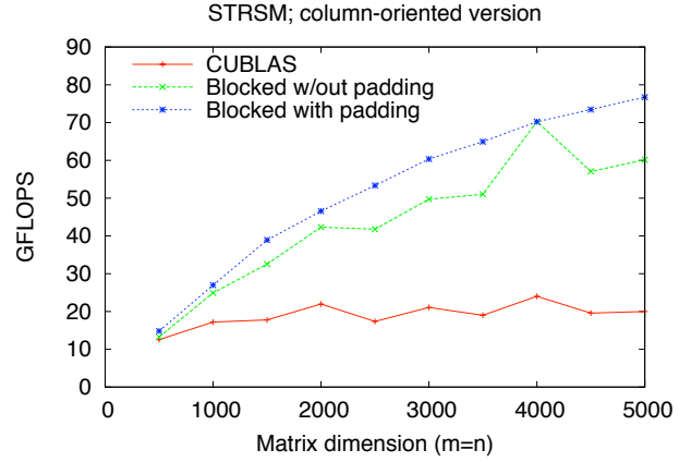
Figure 10. Performance evaluation of the column-oriented blocked implementation of STRSM built on top of SGEMM
