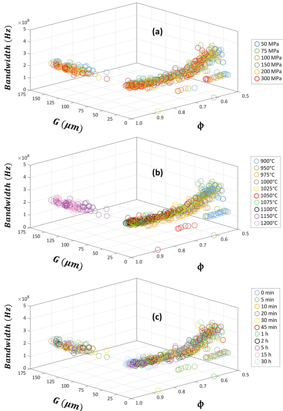
Fig. 8 – Sintered microstructure (relative density \phi and average grain size G ) dependence of bandwidth for RL \leq -20\text{dB} of the sintered Cu-doped Ni-Zn-polycrystalline ferrite: effect of pressing pressure P (a), sintering temperature T (b) and sintering time t (c).
