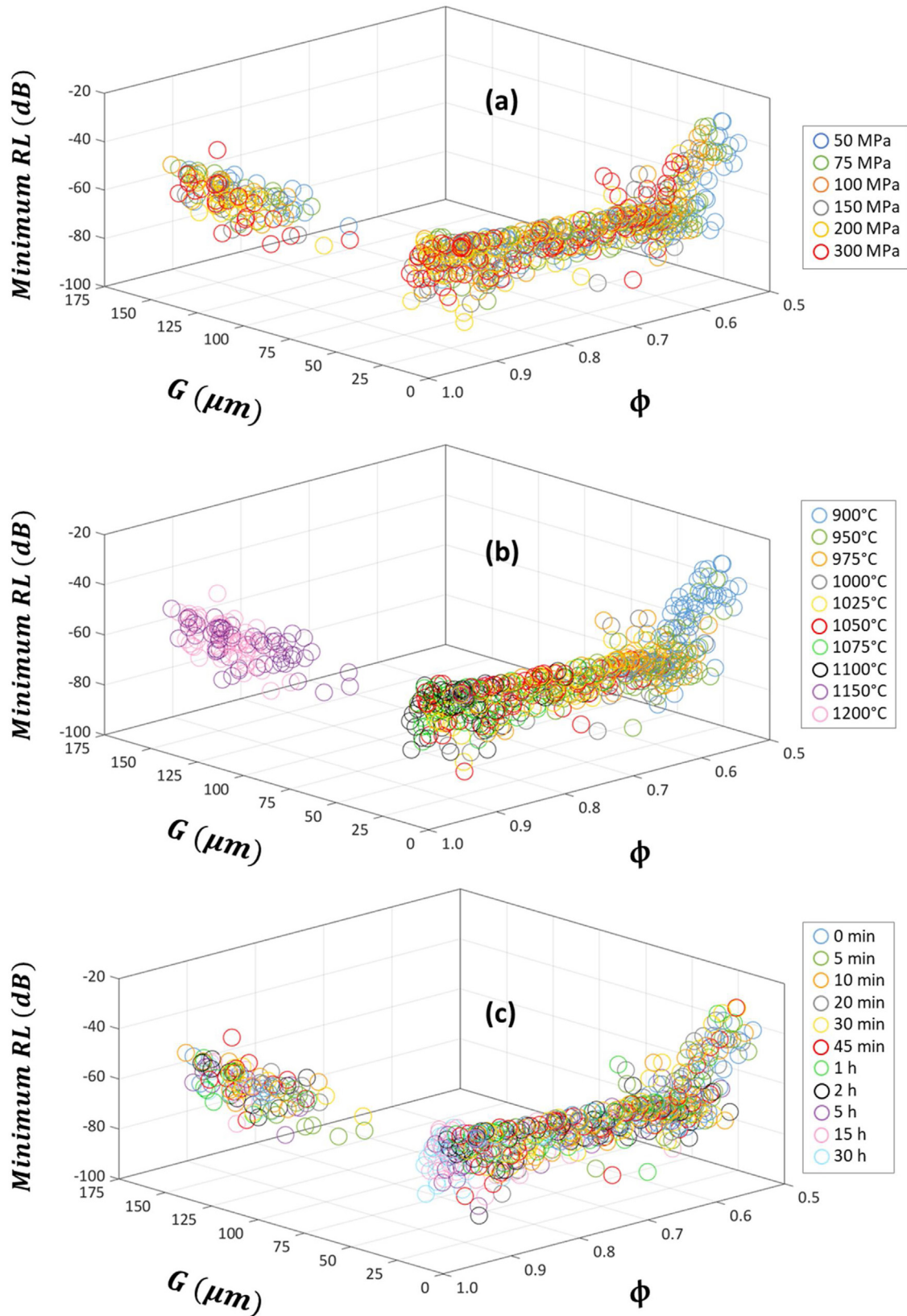
Fig. 9 – Sintered microstructure (relative density \phi and average grain size G ) dependence of minimum reflection loss RL of the sintered Cu-doped Ni-Zn-polycrystalline ferrite: effect of pressing pressure P (a), sintering temperature T (b) and sintering time t (c).
