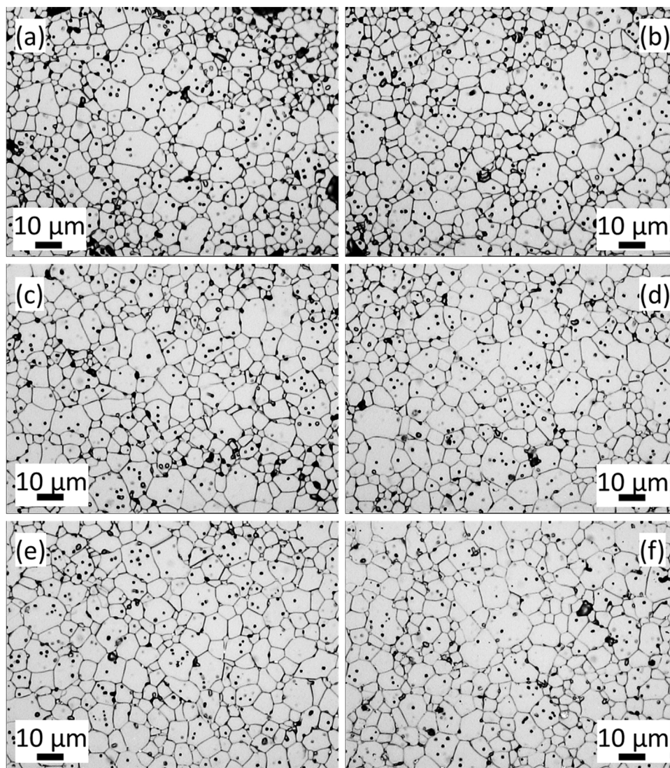
Fig. 2 – SEM images of the polished and etched cross-section areas of the sintered specimens uniaxially pressed at 50 (a), 75 (b), 100 (c), 150 (d), 200 (e) and 300 MPa (f) ( T = 1100^\circ\text{C} and t = 30 min).
