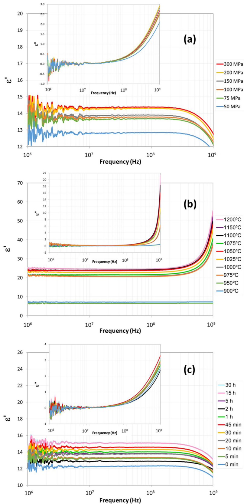
Fig. 4 – Frequency dependence of real \epsilon' and imaginary \epsilon'' parts of complex relative permittivity \epsilon^* of the sintered Cu-doped Ni-Zn-polycrystalline ferrite. Effect of pressing pressure P (a), sintering temperature T (b) and sintering time t (c).
