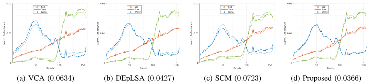
Fig. 1. Qualitative endmember assessment for the four best methods over the Samson dataset. Note that the corresponding ground-truth spectral signatures are plotted using dashed lines and the obtained SAD results are provided in brackets.
