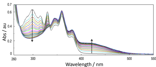
Figure 3. Photooxidation of DHN by ^1\text{O}_2 induced by irradiation of 1 in \text{CH}_3\text{CN} , monitored by UV-Vis spectroscopy. [\text{DHN}] = 80 \mu\text{M} ; [\mathbf{1}] = 33 \mu\text{M} .
