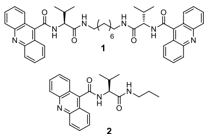
Figure 1. Synthesized compounds based on the 9-amidoacridine chromophore.
