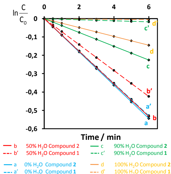
Figure 4. Comparison of pseudo-first order linear fitting for the production of singlet oxygen of 1 and 2 in different media (CH 3 CN/H 2 O).
