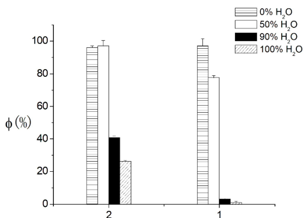
Figure 5. Singlet oxygen generation quantum yield ( \Phi_{\Delta} ) of compound 2 and 1 in different media (CH 3 CN/H 2 O).
