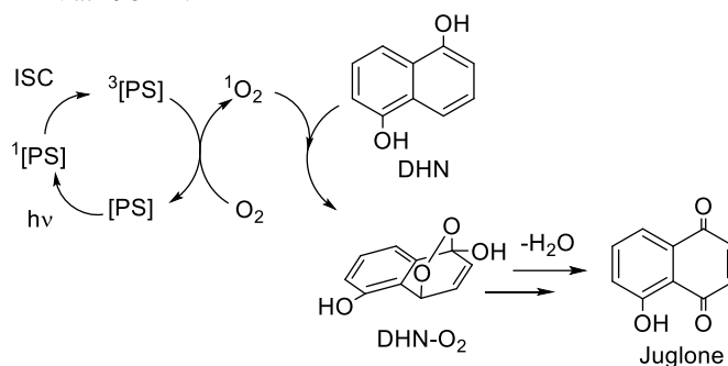
Scheme 2. Photooxidation reaction of DHN. PS = Acridine photosensitizer; ISC = Intersystem crossing; DHN = 1,5-dihydroxynaphthalene.
