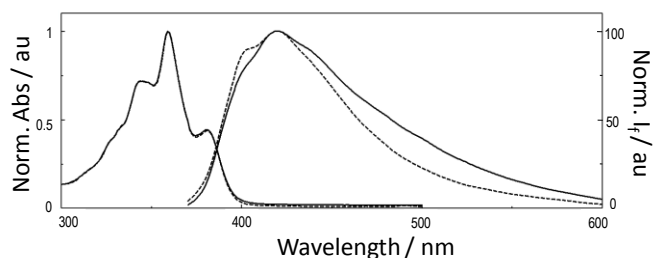
Figure 2. Absorption and emission spectra of synthesized compounds in \text{CH}_3\text{CN} . 1 continuous line, 2 dashed line.
