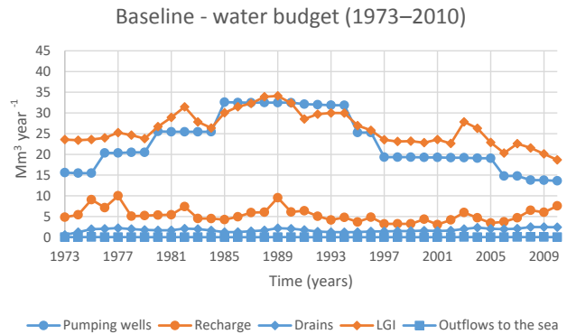
Figure 10. Historical evolution of inflows and outflows in the aquifer.
