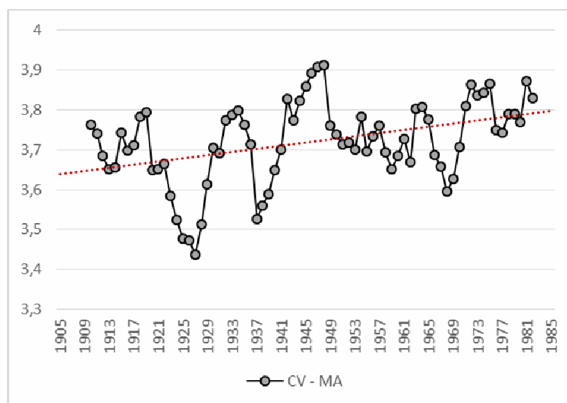
Figure 5. Coefficients of variation (CV, trend). Hellín, 1908-1985
