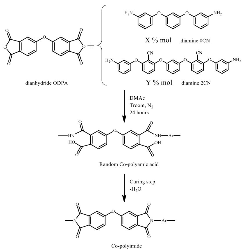
Figure 2 - Scheme of the two-step reaction used for the synthesis of the co-polyamines
