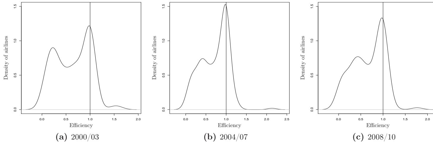
Figure 5: Kernel density plots, efficiency scores (intermediate)
