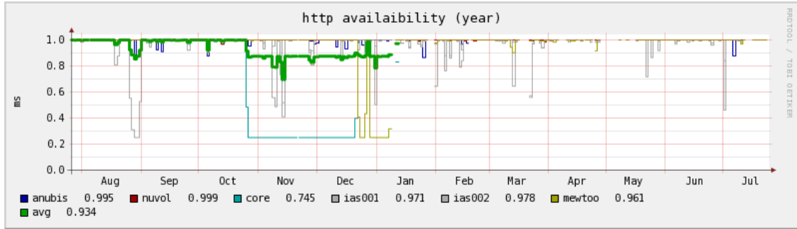
http availability (year)
