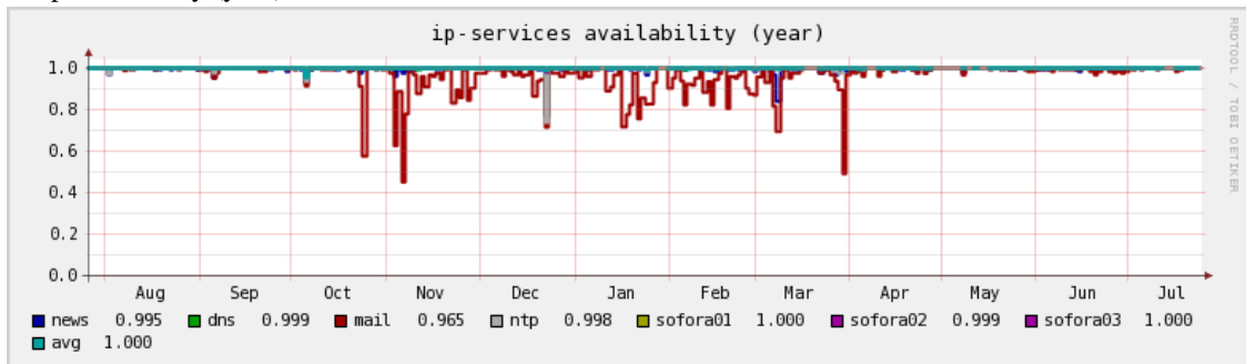
ip-services availability (year)
