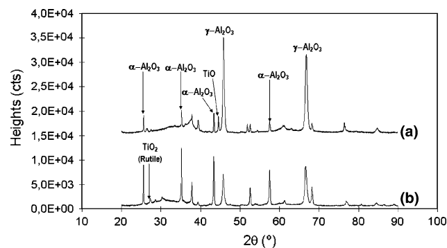
Fig. 4 XRD patterns of \text{Al}_2\text{O}_3 - \text{TiO}_2 plasma-sprayed coatings (standard spraying parameters, see Table 2) using (a) conventional or (b) nanostructured powders
