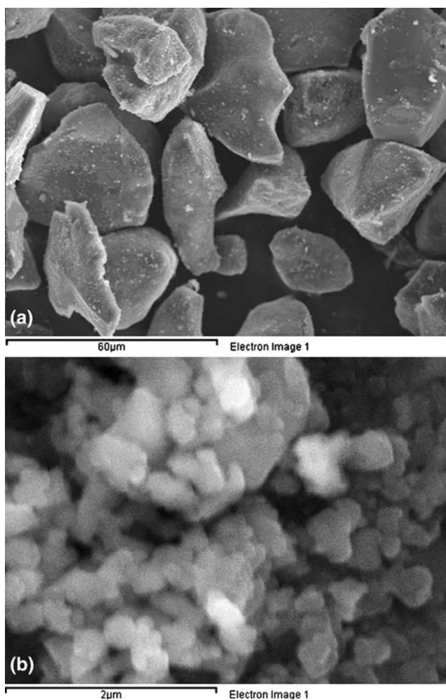
Fig. 2 SEM micrographs of (a) conventional and (b) nanostructured \text{Al}_2\text{O}_3 -13wt.% \text{TiO}_2 thermal spray powders (secondary electron mode)
