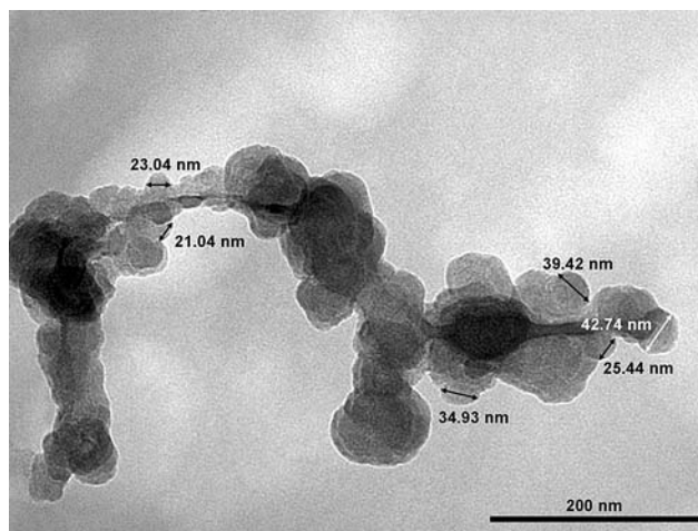
Fig. 3 TEM micrograph of the nanostructured \text{Al}_2\text{O}_3 -13wt.% \text{TiO}_2 thermal spray powder
