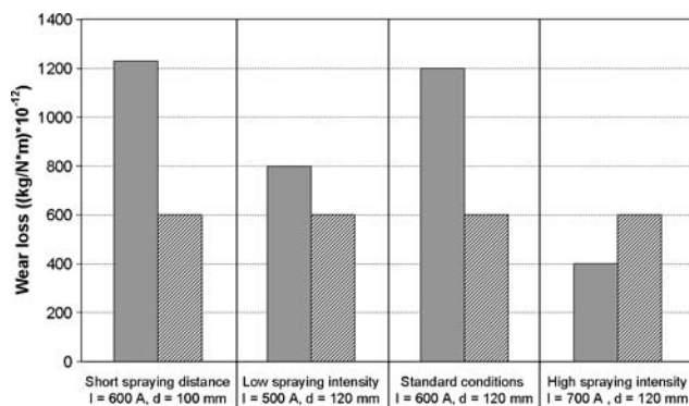
Fig. 13 Wear loss of conventional coatings (grey columns) and nanostructured coatings (striped columns) determined by pin-on-disc experiments
