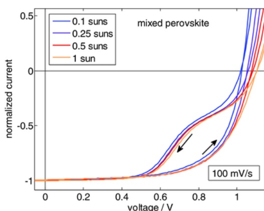
Figure 28. Inverted hysteresis in J - V curves of mixed perovskite-based devices at different illumination intensities. Reprinted with permission. [125] Copyright 2016, John Wiley & Sons.
