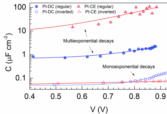
Figure 18. Capacitance as function of V_{oc} from PI-DC (circles) and PI-CE (triangles) for two devices: \text{TiO}_2/\text{MAPbI}_3/\text{spiro-OMeTAD} (filled dots) and \text{PEDOT}/\text{MAPbI}_3/\text{PCBM} (open dots). A clear difference between techniques arises when multiexponential decays occur. Data courtesy of Emilio Palomares.
