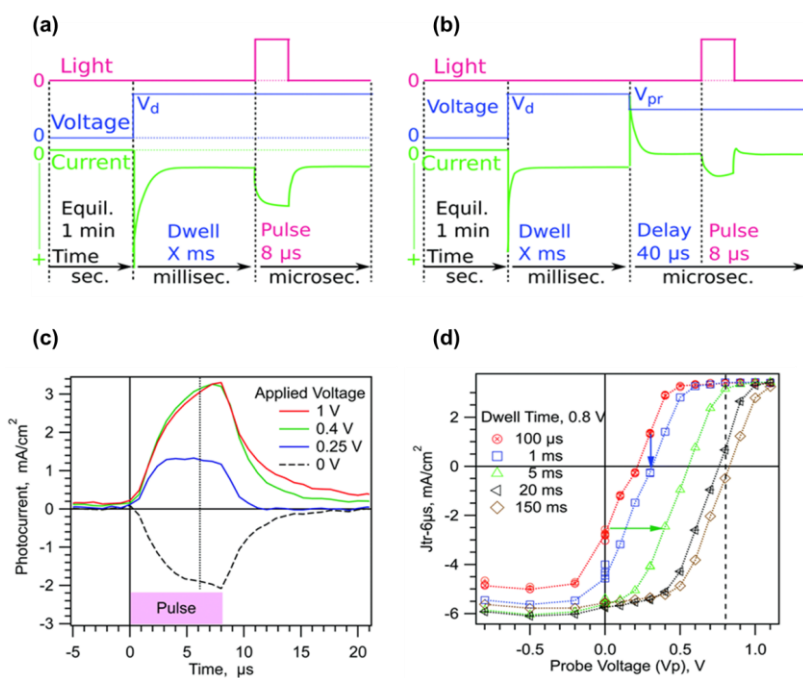
Figure 27. Schematic of (a) step-dwell-probe (SDP) method and (b) step-dwell-step-probe (SDSP) method with corresponding timescales shown. (c) shows the current transients for different step voltages V_d in a SDP experiment on planar \text{MAPbI}_3 samples. (d) shows the corresponding SDSP measurement for the same sample for different dwell times as shown in the legend. Adapted with permission. [9] Copyright 2017, Royal Society of Chemistry.
