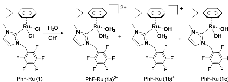
Scheme 3. Aqueous chemical speciation of PhF-Ru ( 1 ).
