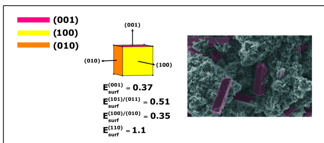
Figure 6. SEM image of cubic anatase TiO 2 particle and its Wulff crystal representation. Surface energy is in joule per-square meter.
