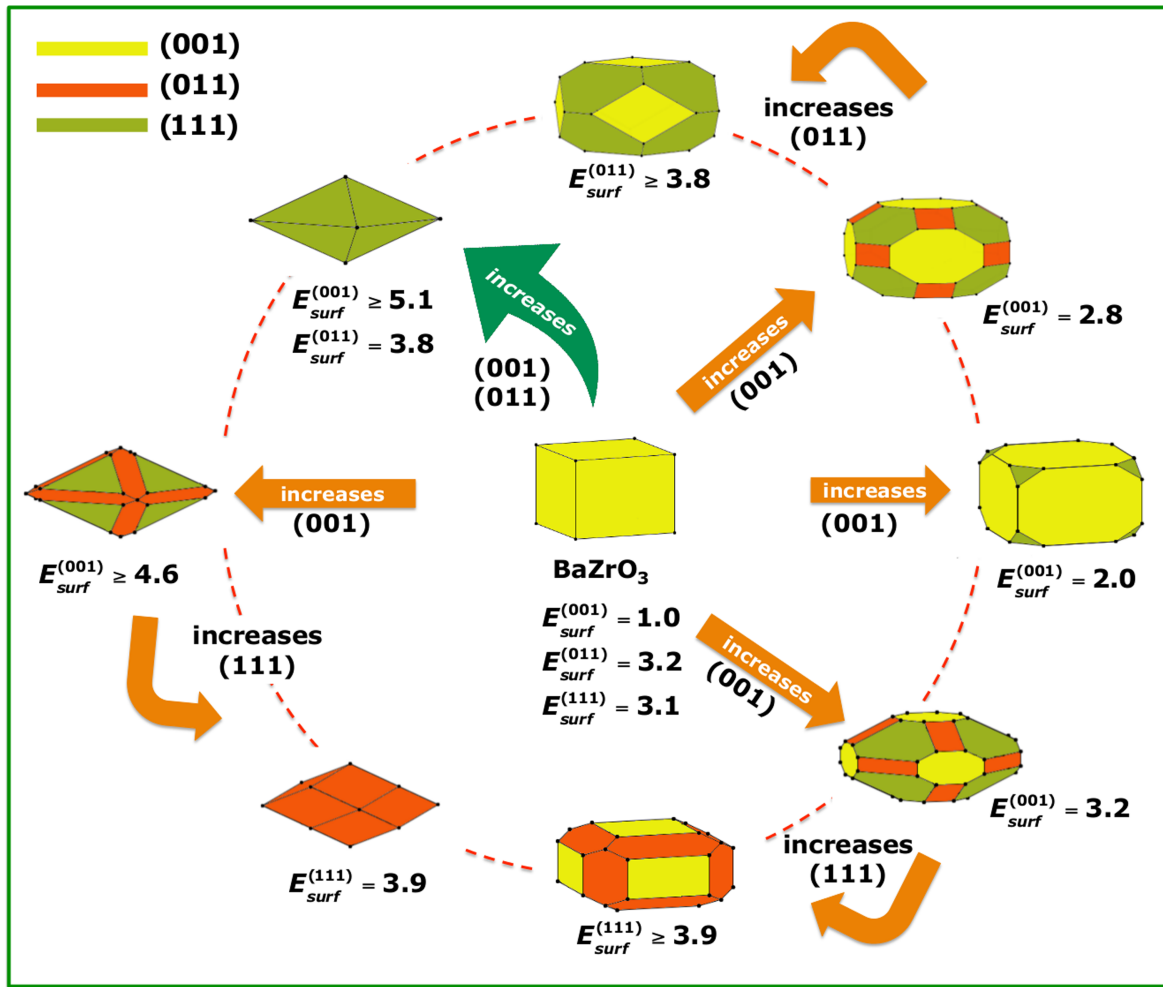
Figure 8. Crystallographic structure and map of morphologies of BaZrO 3 with (001), (011), and (111) crystal planes. Surface energy is in joule per-square meter. Theoretical (experimental) [130] lattice parameter, a = 4.251 \text{ \AA} ( 4.18 \text{ \AA} ).
