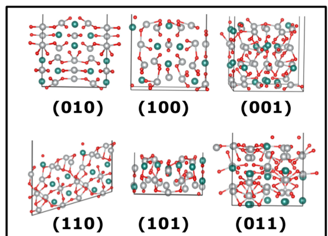
Figure 10. Surface models of (010), (100), (001), (110), (101), and (011) for \alpha -Ag 2 WO 4 . The Ag, W, and O atoms appear in gray, blue, and red, respectively.
