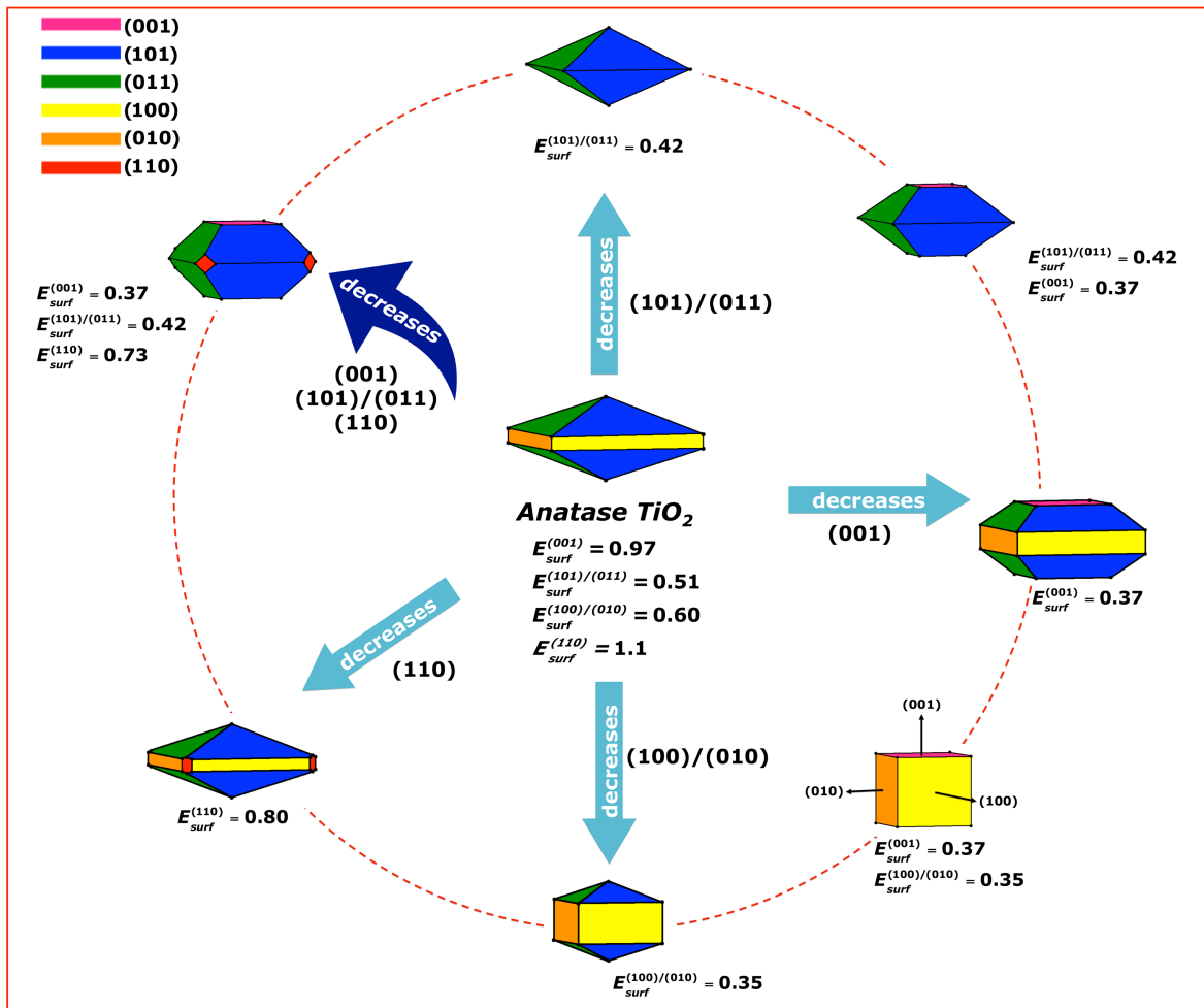
Figure 5. Crystallographic structure and map of morphologies of anatase TiO 2 with crystal planes (001), (101), (011), (100), (010), and (110). Surface energy is in joule per-square meter. Theoretical (experimental) [120] lattice parameters, a = 3.806 \text{ \AA} (3.78 Å), c = 9.722 \text{ \AA} (9.51 Å).
