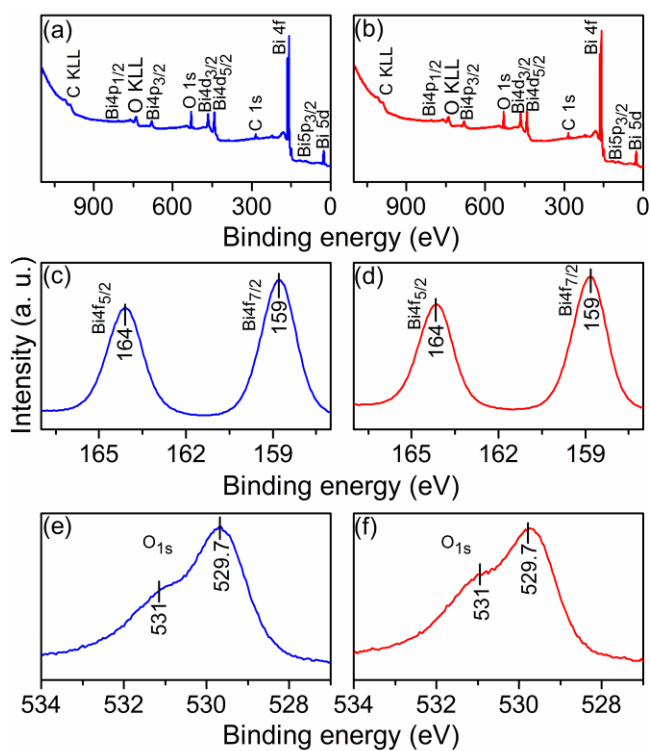
Figure 8. XPS spectra of samples (a) \alpha\text{-Bi}_2\text{O}_3\text{-MAH} and (b) \alpha\text{-Bi}_2\text{O}_3\text{-PAHT} . XPS spectra of \text{Bi}4f_{7/2} and \text{Bi}4f_{5/2} levels for (c) \alpha\text{-Bi}_2\text{O}_3\text{-MAH} and (d) \alpha\text{-Bi}_2\text{O}_3\text{-PAHT} . XPS spectra of \text{O}1s levels for (e) \alpha\text{-Bi}_2\text{O}_3\text{-MAH} and (f) \alpha\text{-Bi}_2\text{O}_3\text{-PAHT} .
