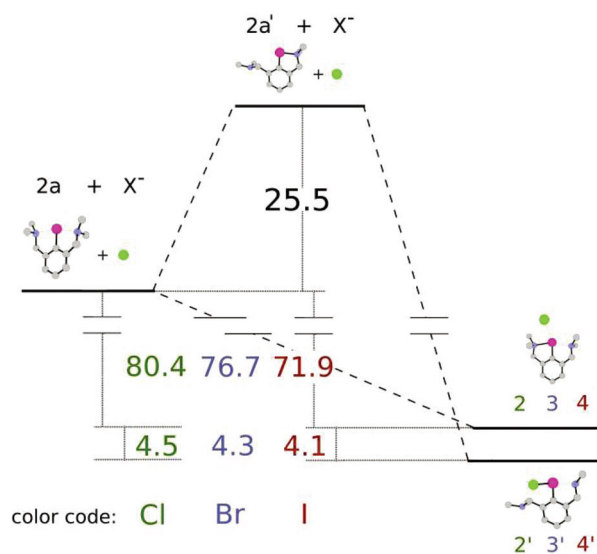
Fig. 6 Enthalpy of formation ( \Delta H_f^{298} , kcal mol –1 ) for compounds 2–4 starting from 2a , and for compounds 2'–4' starting from 2a via the intermediate cation 2a' .
