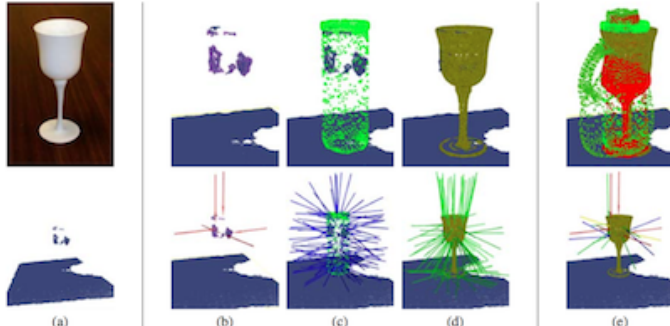
Figure 28: a) Object and point cloud. b,c,d) Object representation and grasp hypotheses. e) Overlaid representations and list of consistent grasp hypotheses [62, 130].
